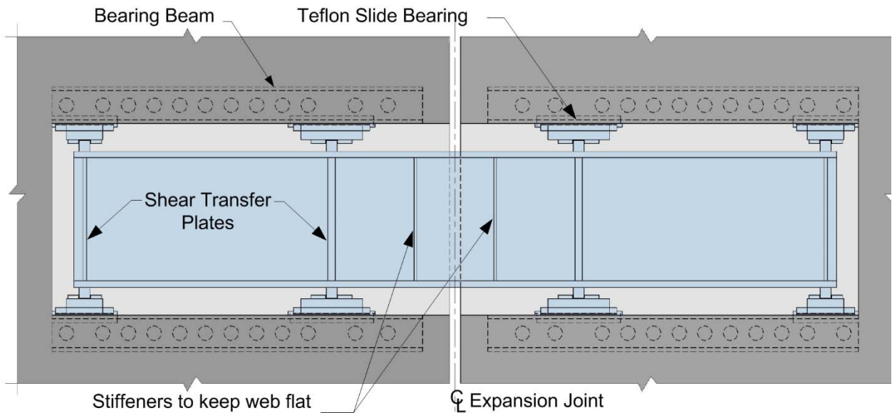
Beam Installation
