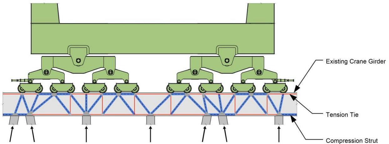
Figure 6. Strut-and-tie girder analysis
