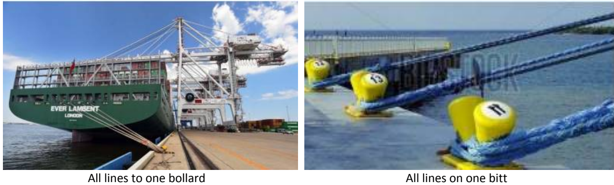
Figure 5. Suboptimal mooring line arrangements
